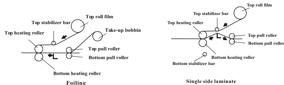
Film Threading Diagram
